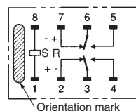
Terminal arrangement/ Internal connections
