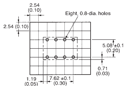
Mounting pads (top view)
