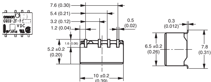
Terminal arrangement/ Internal connections (top view)
