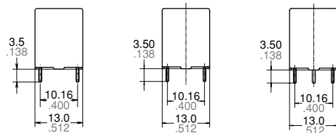
Single side stable type 1 coil latching type 2 coil latching type
