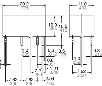
2 coil latching
