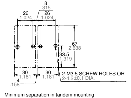
Layout for tandem mounting
