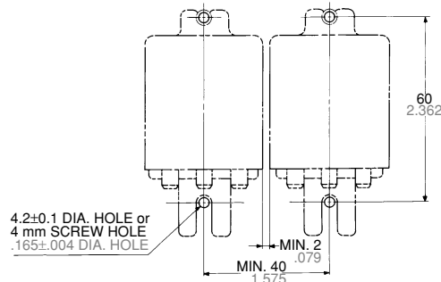
Mounting dimension
