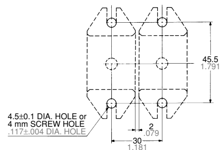
Mounting dimensions
