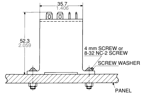
Mounting dimensions
