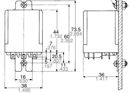
4 mm SCREW or 8-32 NC-2 SCREW SPRING WASHER
