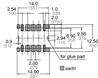
2 coil latching
