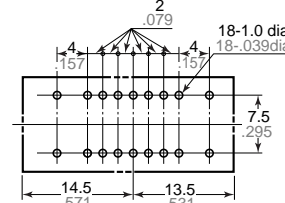
2 coil latching
