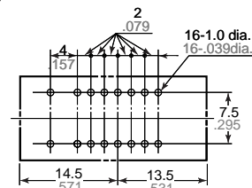
PC board pattern (Bottom view) Single side stable and 1 coil latching
