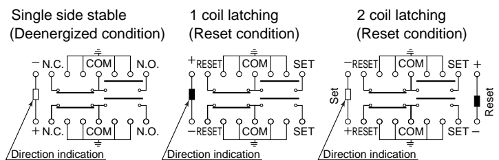
Schematic (Bottom view)
